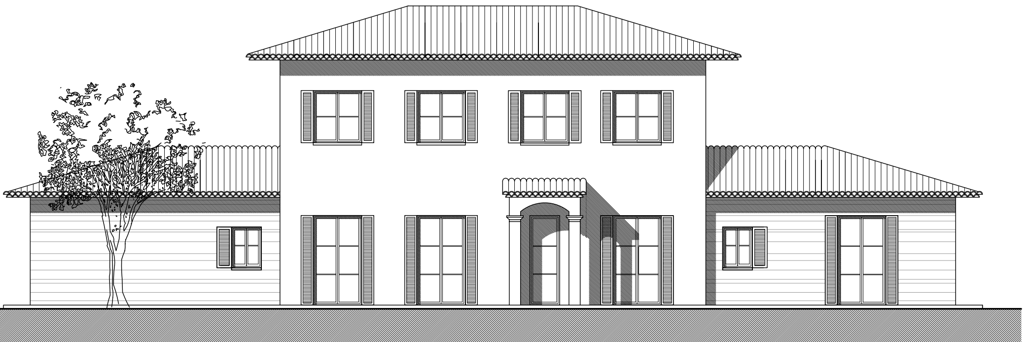
ELEVATION FRONT ENTREE 1 : 100
